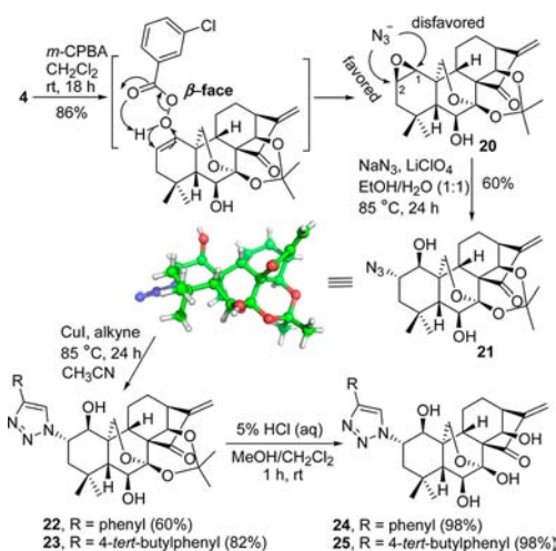
Scheme 3. Synthesis of 2-Azide-, 1,2,3-Triazole-substituted Oridonin Derivatives 21 , 24 and 25
